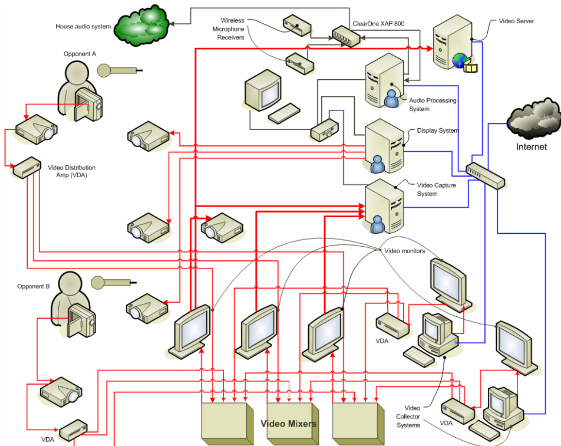
Figure 8 - Utah's Enhanced Performance Grid Node
