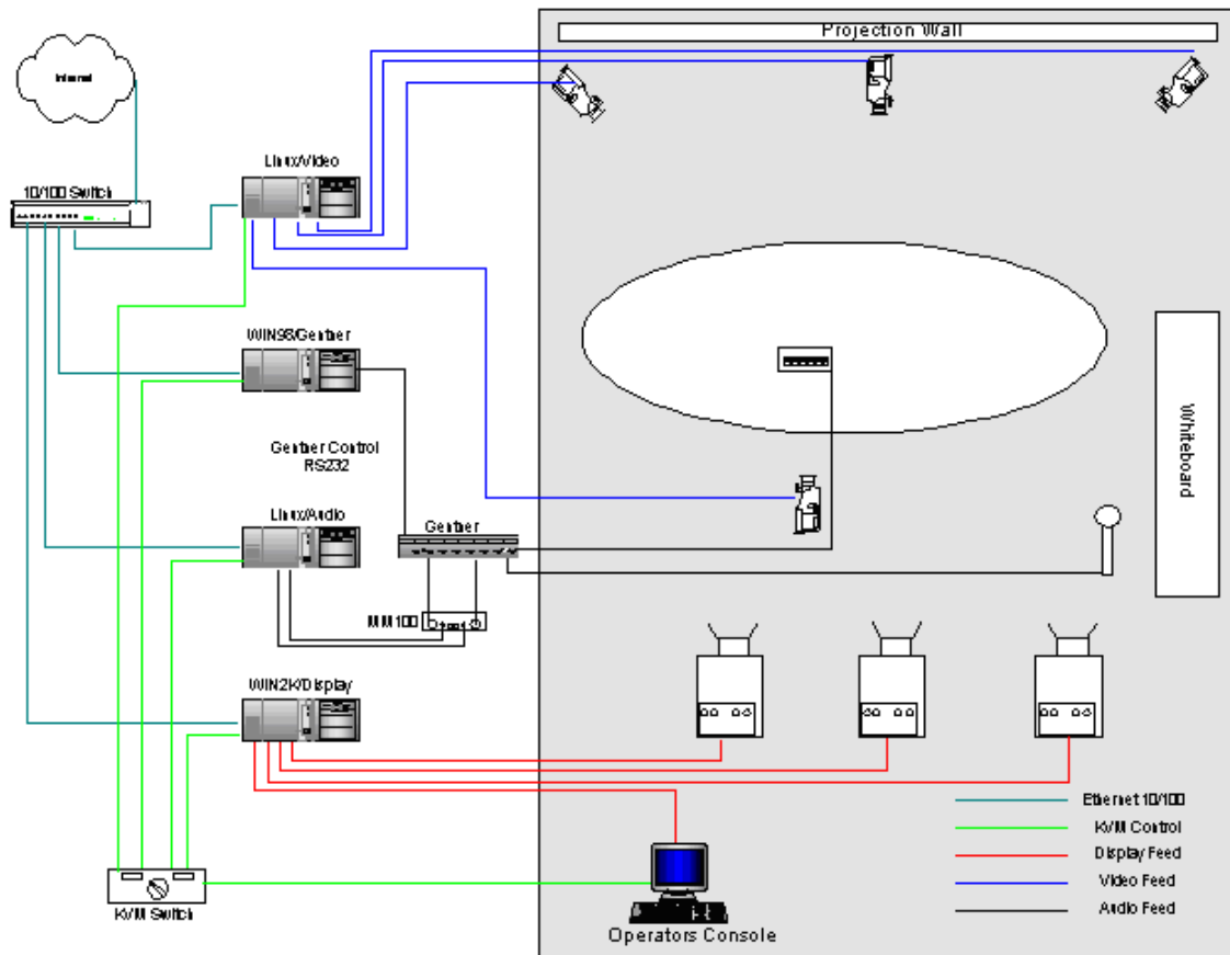
Figure 5 - Basic Access Grid Configuration
